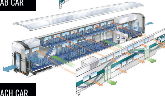
CAB CAR
